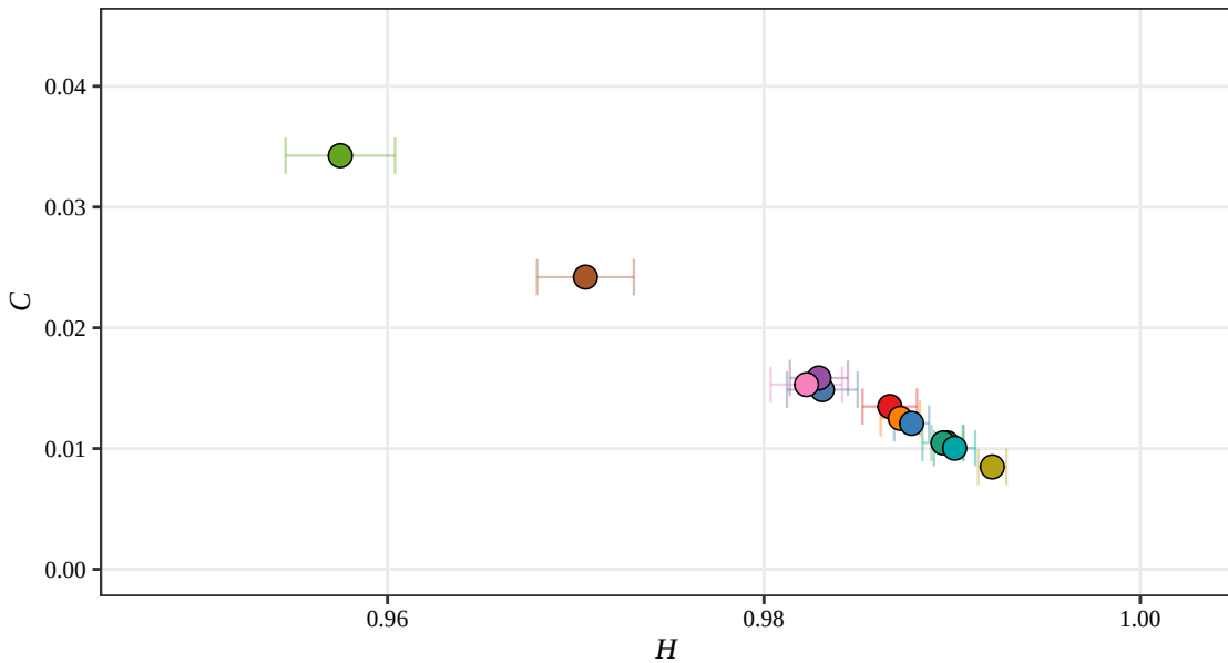
Rényi H-C Plane, D = 5 (Displacement, 2016)
