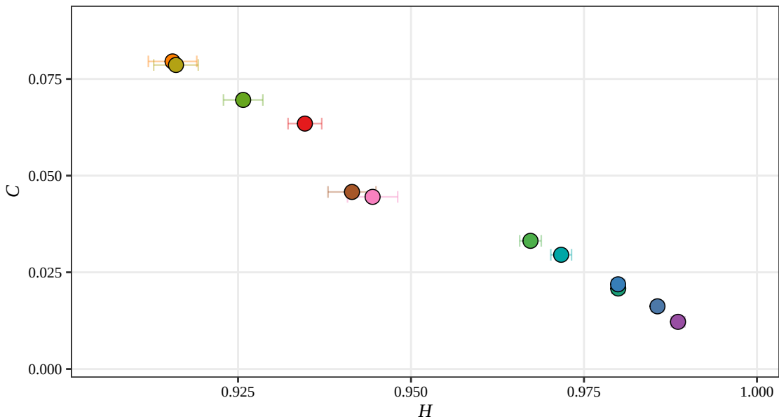
Rényi H-C Plane, D = 5 (RSAM, 2016)
