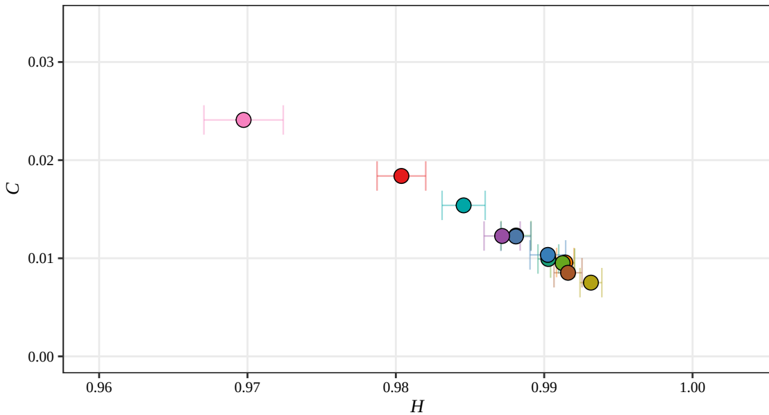
Rényi H-C Plane, D = 5 (Displacement, 2017)
