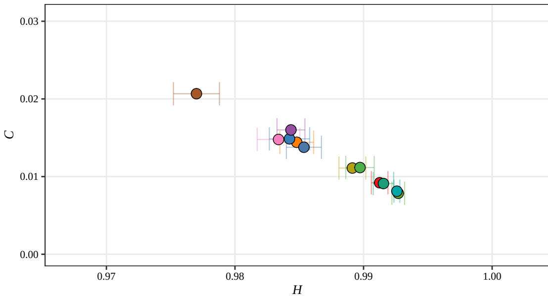
Rényi H-C Plane, D = 5 (Displacement, 2018)
