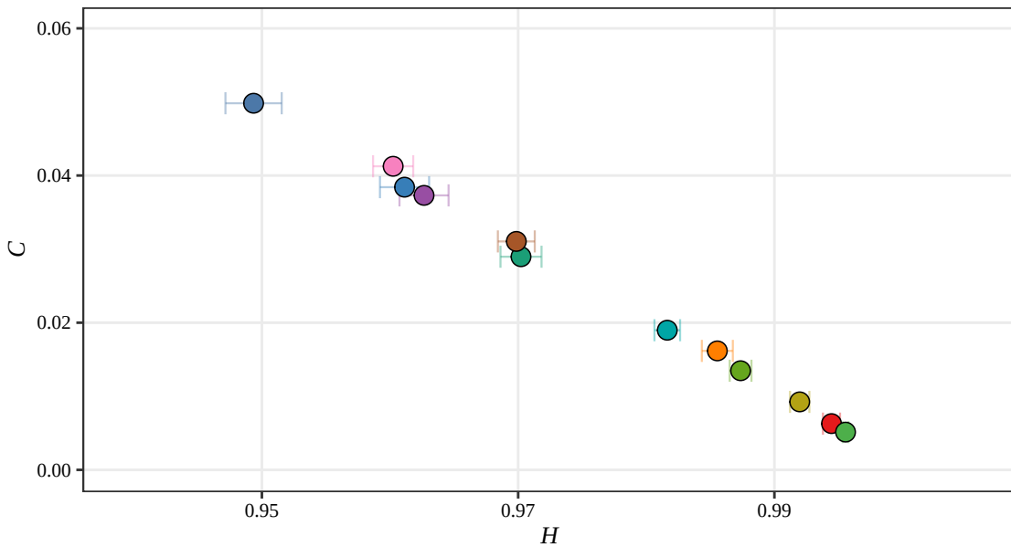
Rényi H-C Plane, D = 5 (RSAM, 2018)
