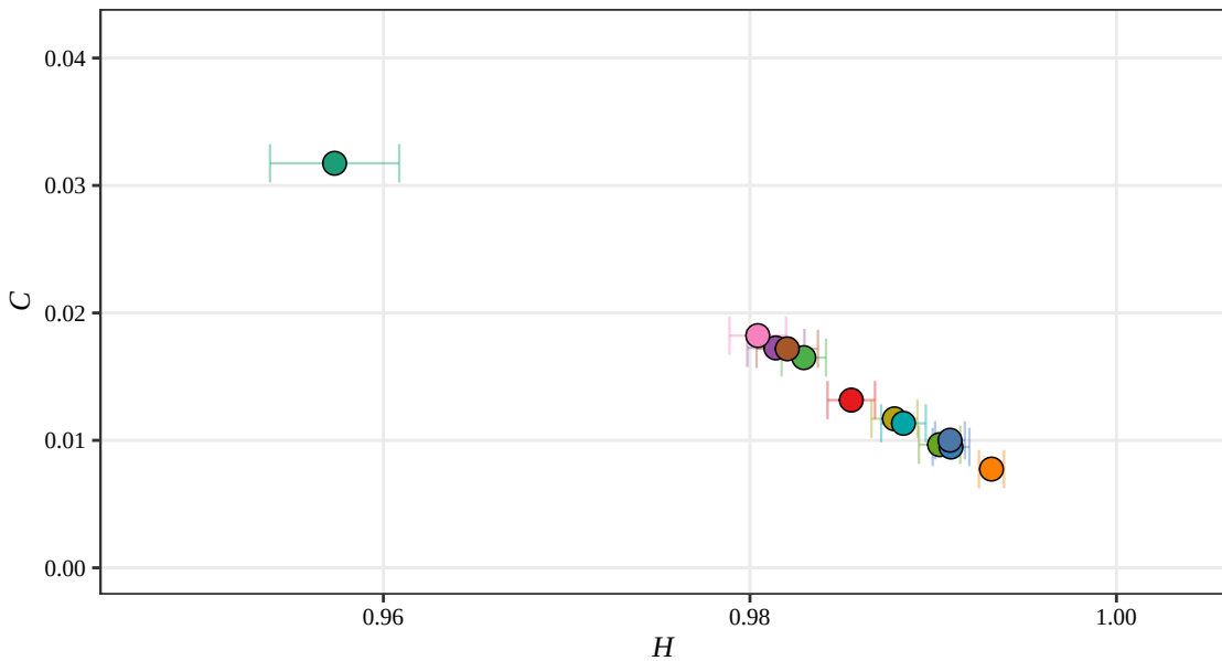
Rényi H-C Plane, D = 5 (Displacement, 2019)
