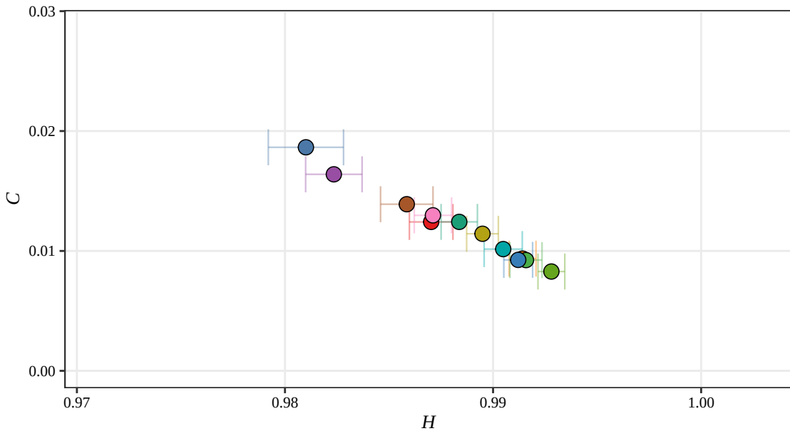
Rényi H-C Plane, D = 5 (Displacement, 2020)
