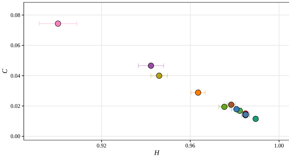
Rényi H-C Plane, D = 5 (Displacement, 2021)
