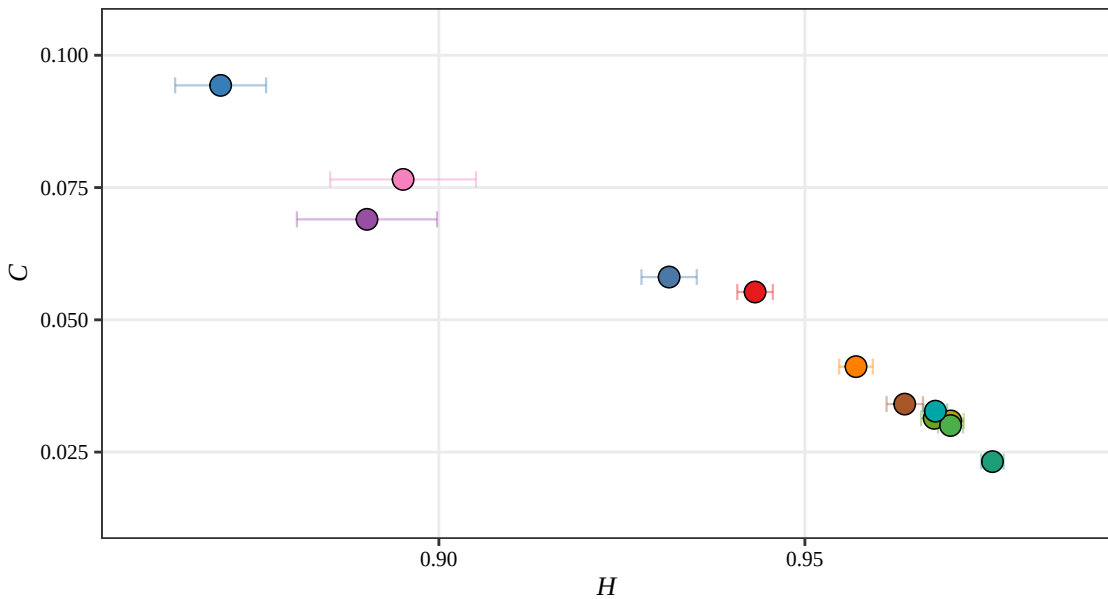
Rényi H-C Plane, D = 5 (RSAM, 2021)
