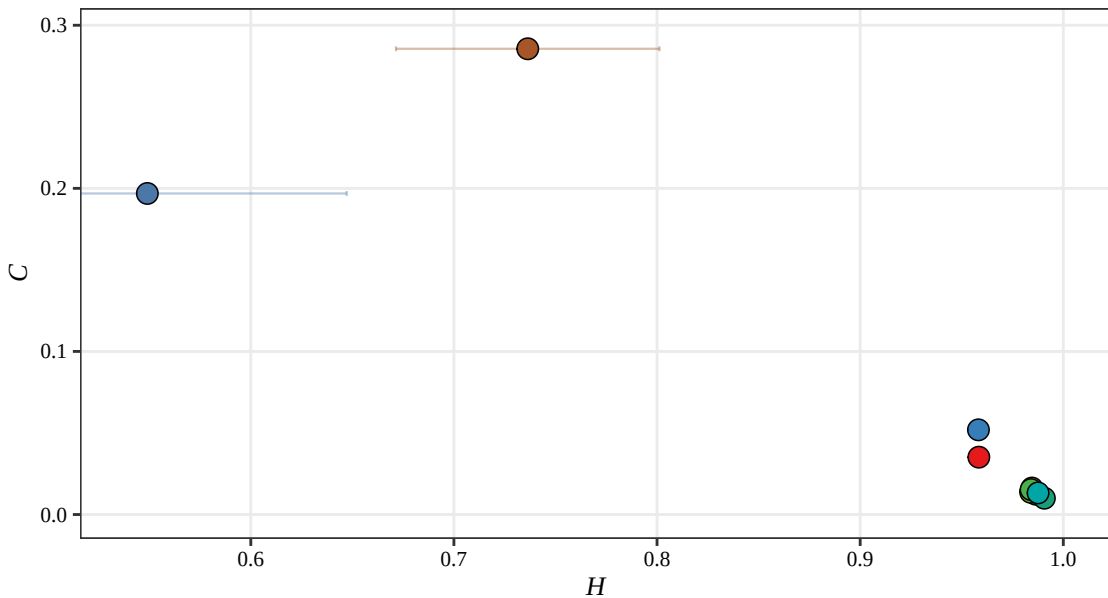
Rényi H-C Plane, D = 5 (Displacement, 2022)
