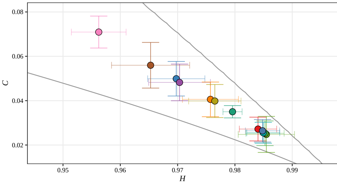
Shannon H-C Plane, D = 5 (RSAM, 2011)
