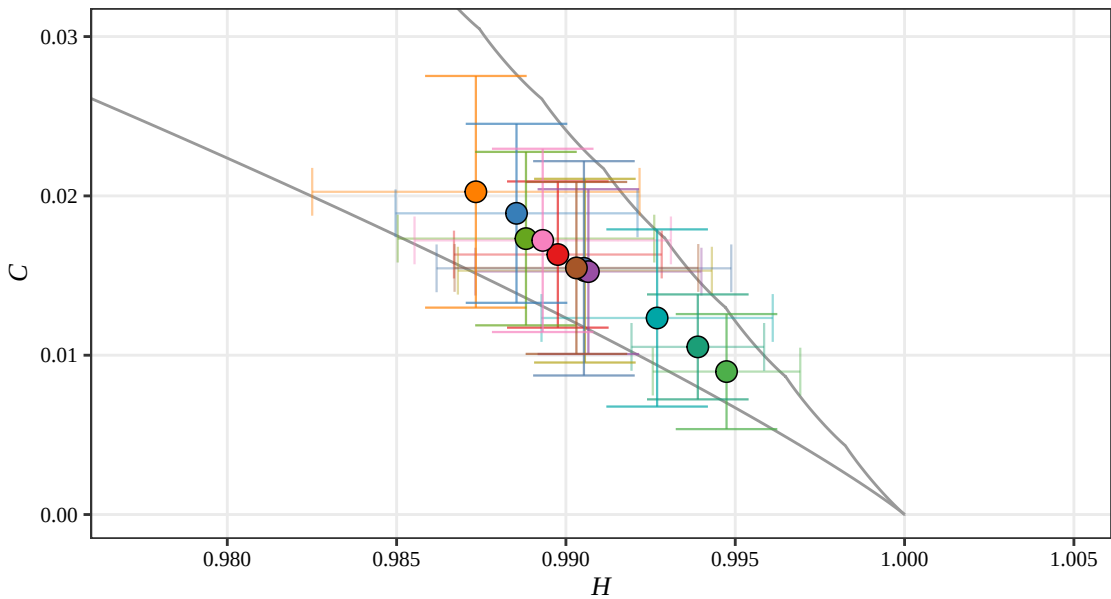
Shannon H-C Plane, D = 5 (Displacement, 2012)
