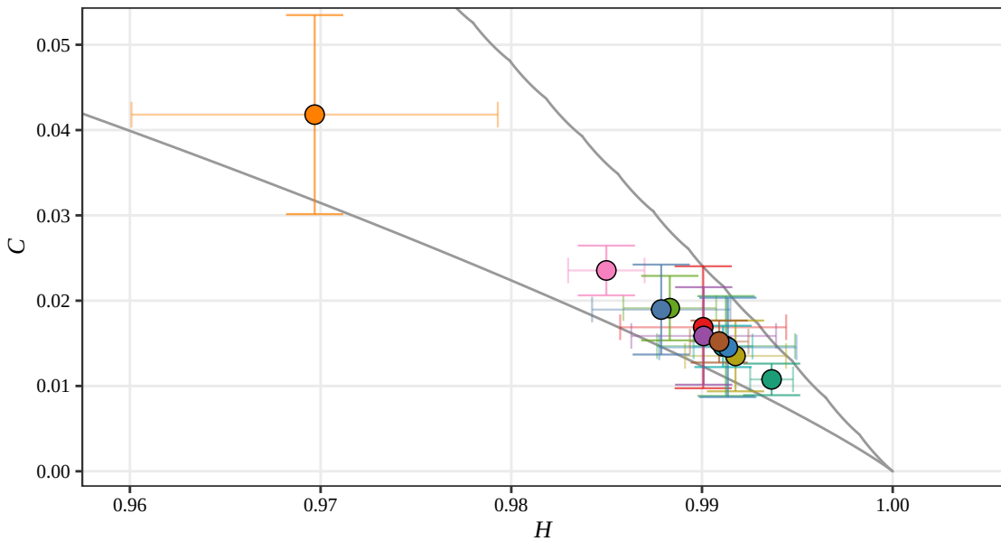
Shannon H-C Plane, D = 5 (Displacement, 2013)
