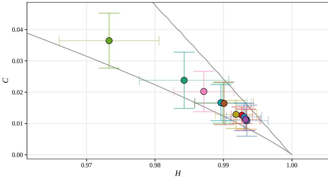
Shannon H-C Plane, D = 5 (Displacement, 2014)
