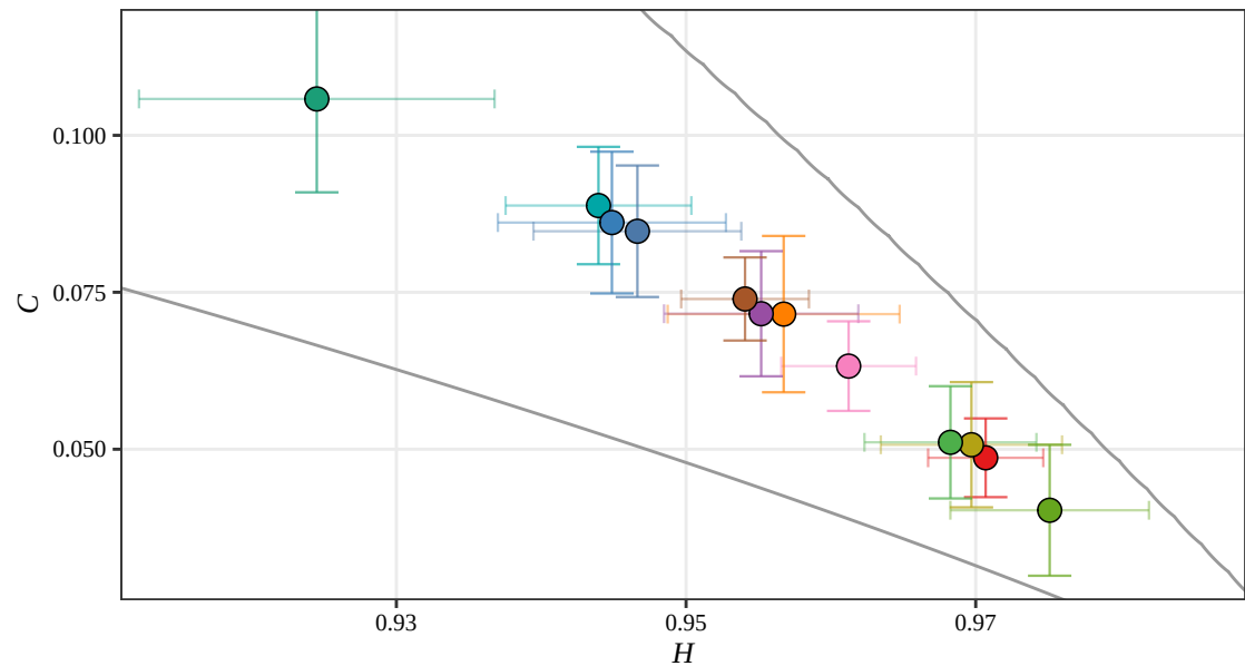
Shannon H-C Plane, D = 5 (RSAM, 2014)
