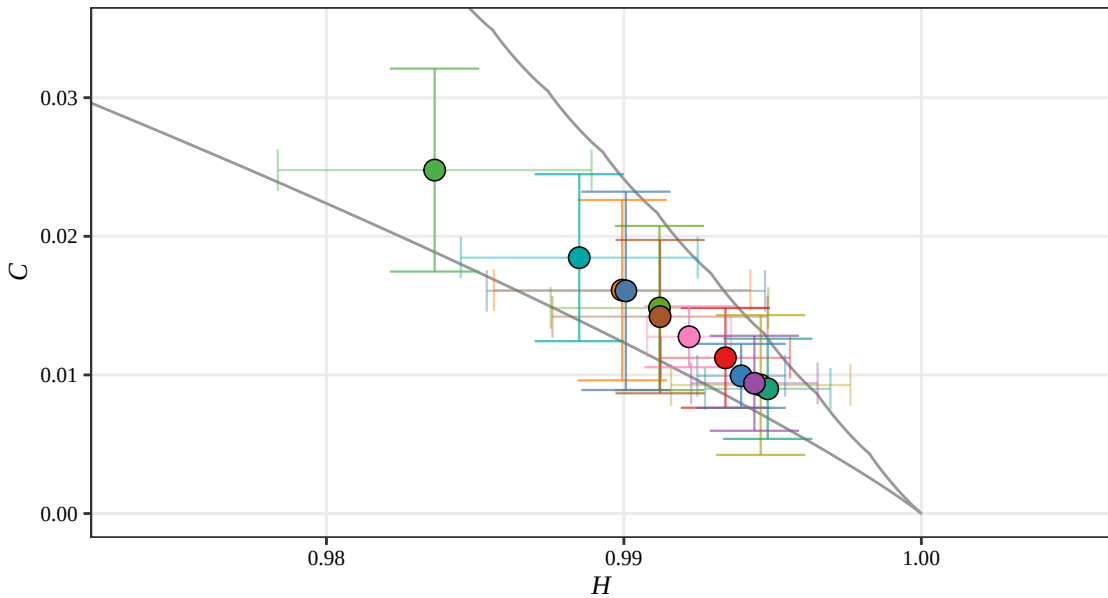
Shannon H-C Plane, D = 5 (Displacement, 2015)
