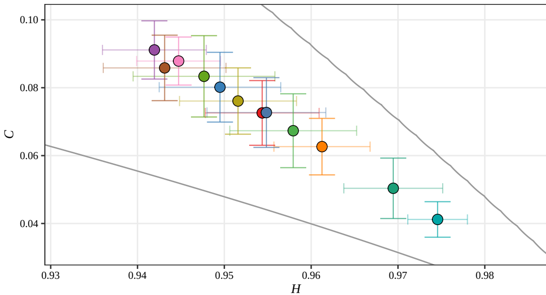
Shannon H-C Plane, D = 5 (RSAM, 2015)
