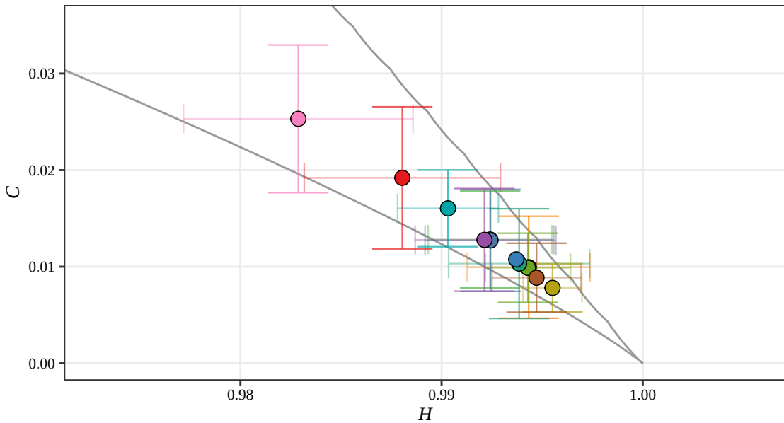
Shannon H-C Plane, D = 5 (Displacement, 2017)
