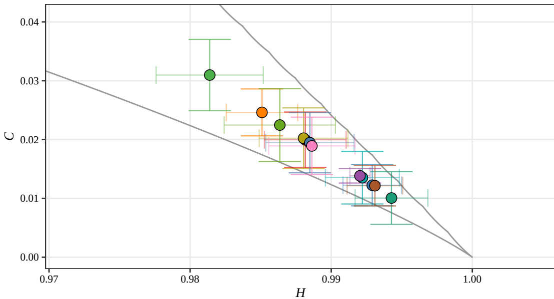
Shannon H-C Plane, D = 5 (RSAM, 2017)
