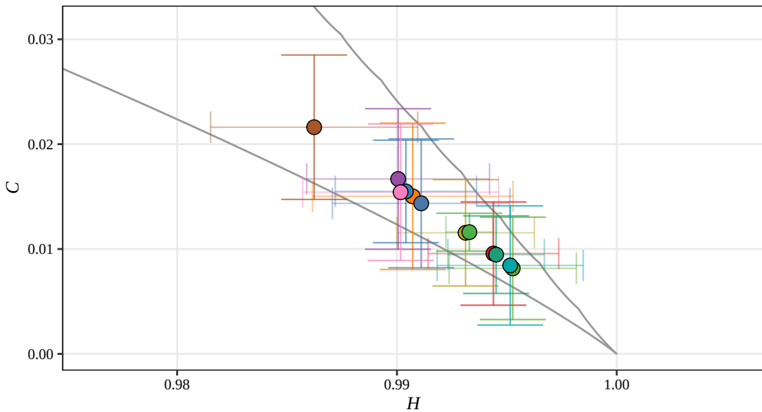
Shannon H-C Plane, D = 5 (Displacement, 2018)
