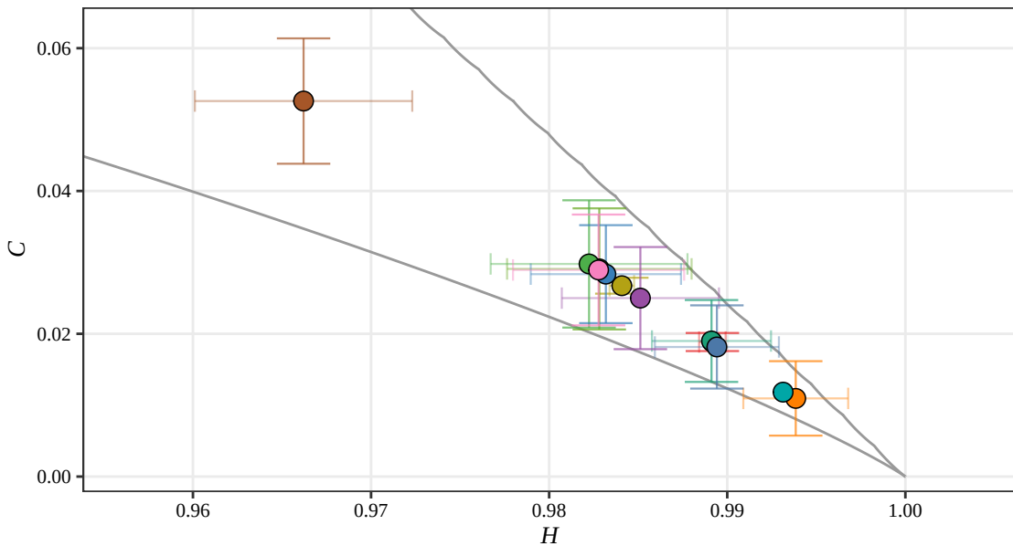
Shannon H-C Plane, D = 5 (RSAM, 2019)
