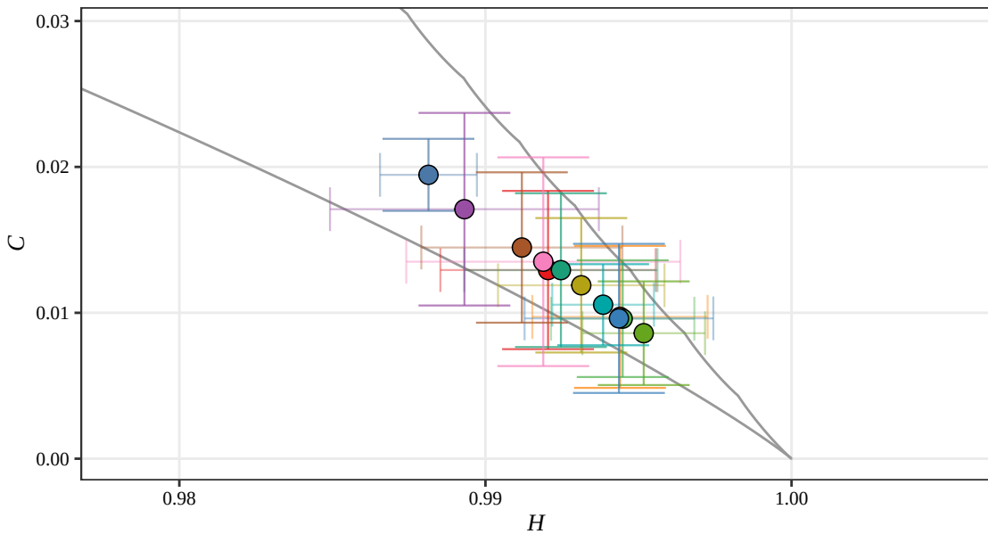
Shannon H-C Plane, D = 5 (Displacement, 2020)
