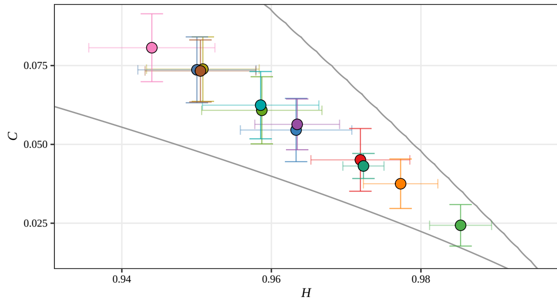
Shannon H-C Plane, D = 5 (RSAM, 2020)
