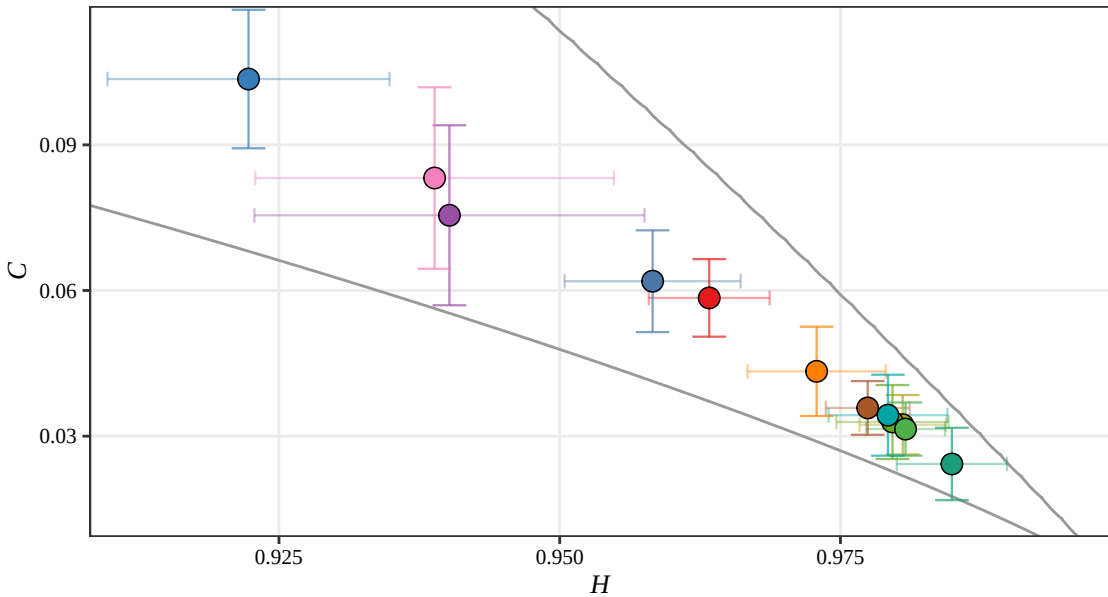
Shannon H-C Plane, D = 5 (RSAM, 2021)
