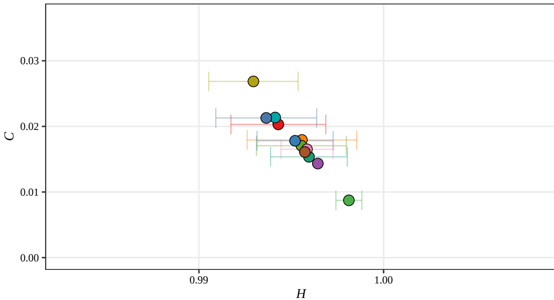
Tsallis H-C Plane, D = 5 (Displacement, 2011)
