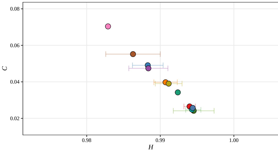
Tsallis H-C Plane, D = 5 (RSAM, 2011)
