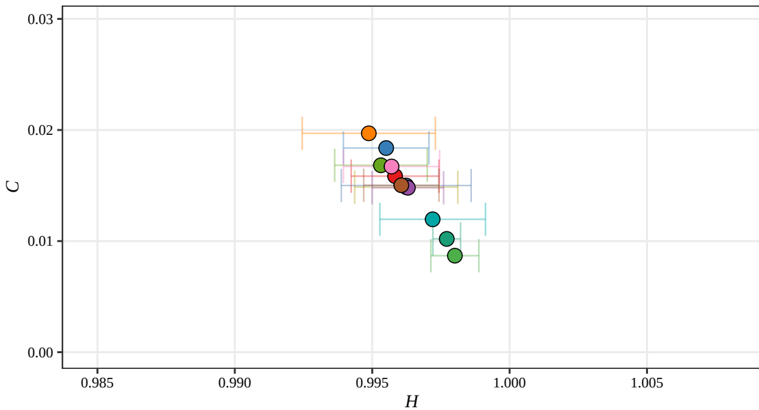
Tsallis H-C Plane, D = 5 (Displacement, 2012)
