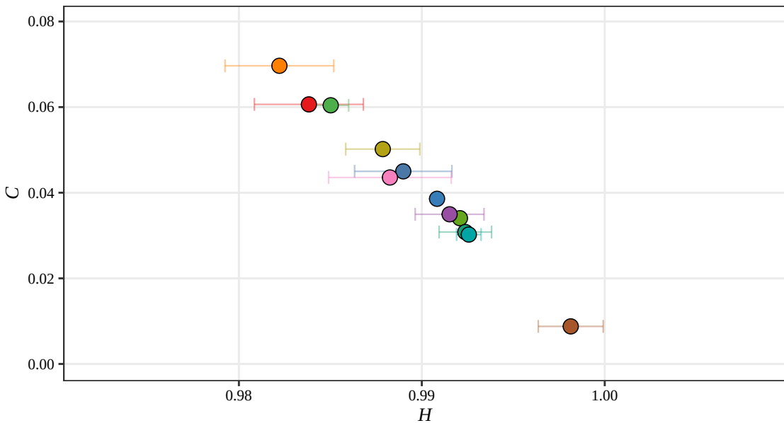
Tsallis H-C Plane, D = 5 (RSAM, 2012)
