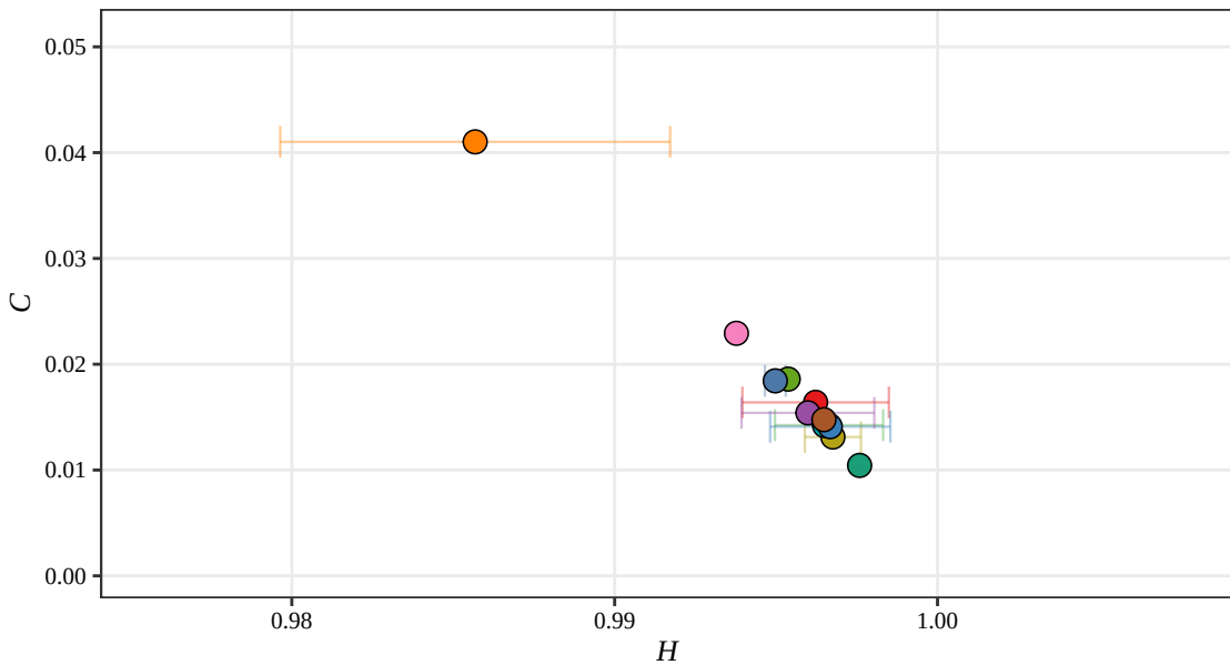
Tsallis H-C Plane, D = 5 (Displacement, 2013)
