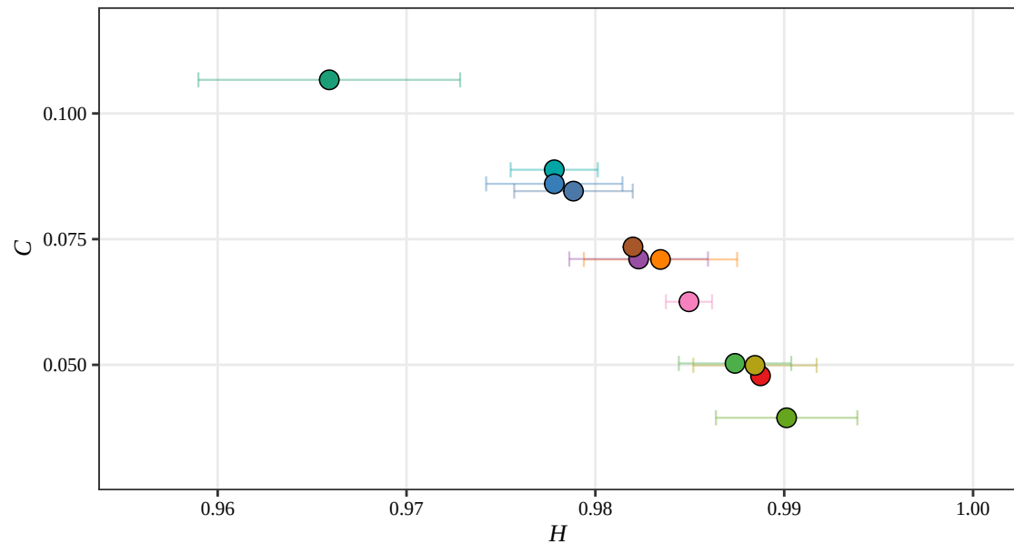
Tsallis H-C Plane, D = 5 (RSAM, 2014)
