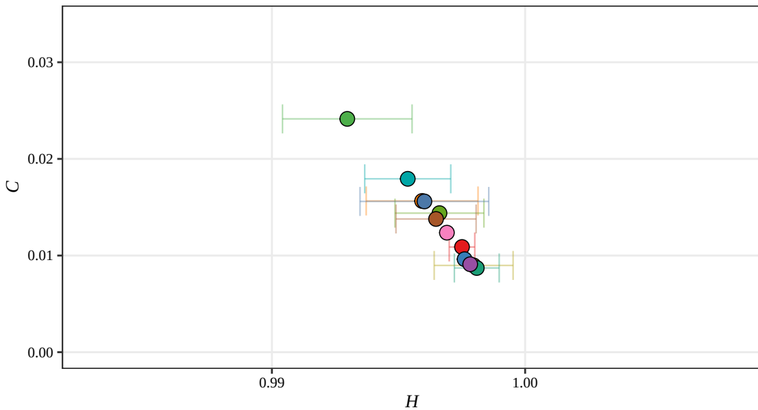
Tsallis H-C Plane, D = 5 (Displacement, 2015)
