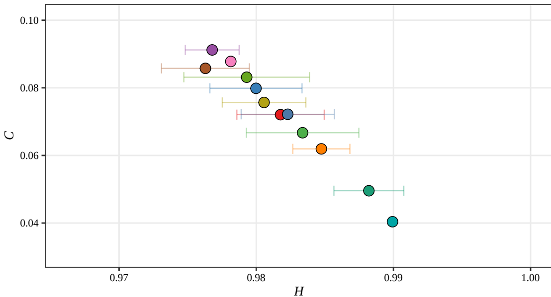
Tsallis H-C Plane, D = 5 (RSAM, 2015)
