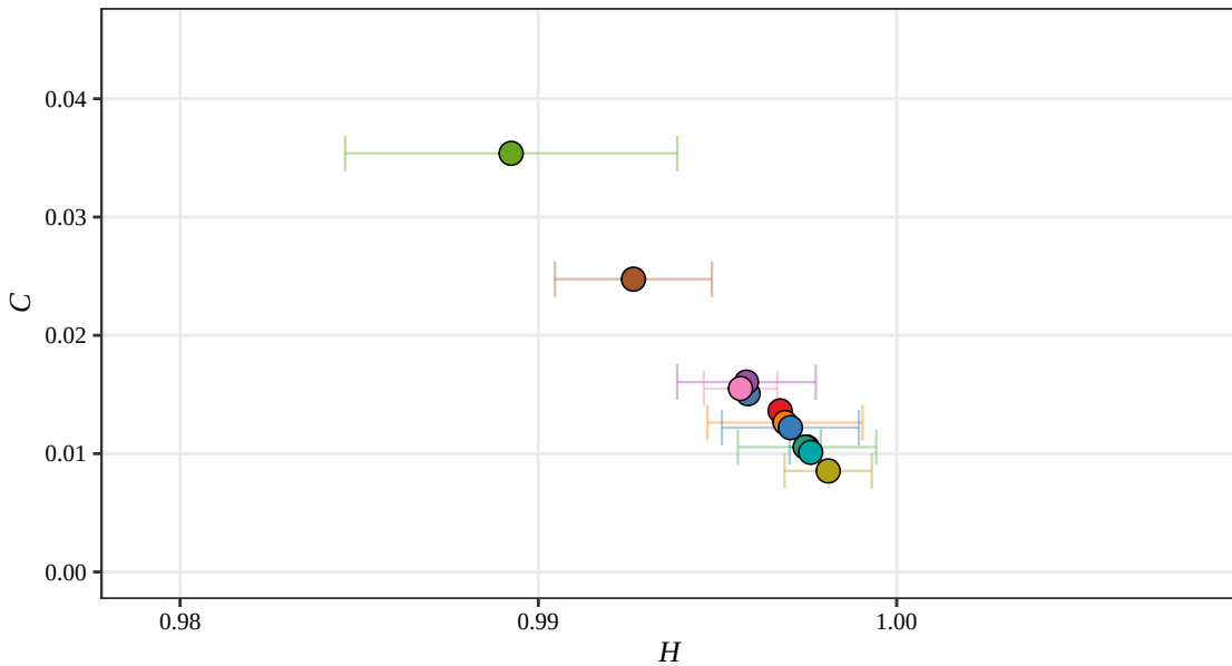
Tsallis H-C Plane, D = 5 (Displacement, 2016)
