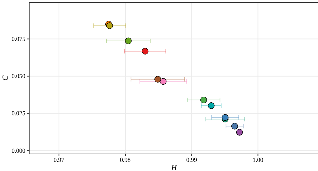
Tsallis H-C Plane, D = 5 (RSAM, 2016)
