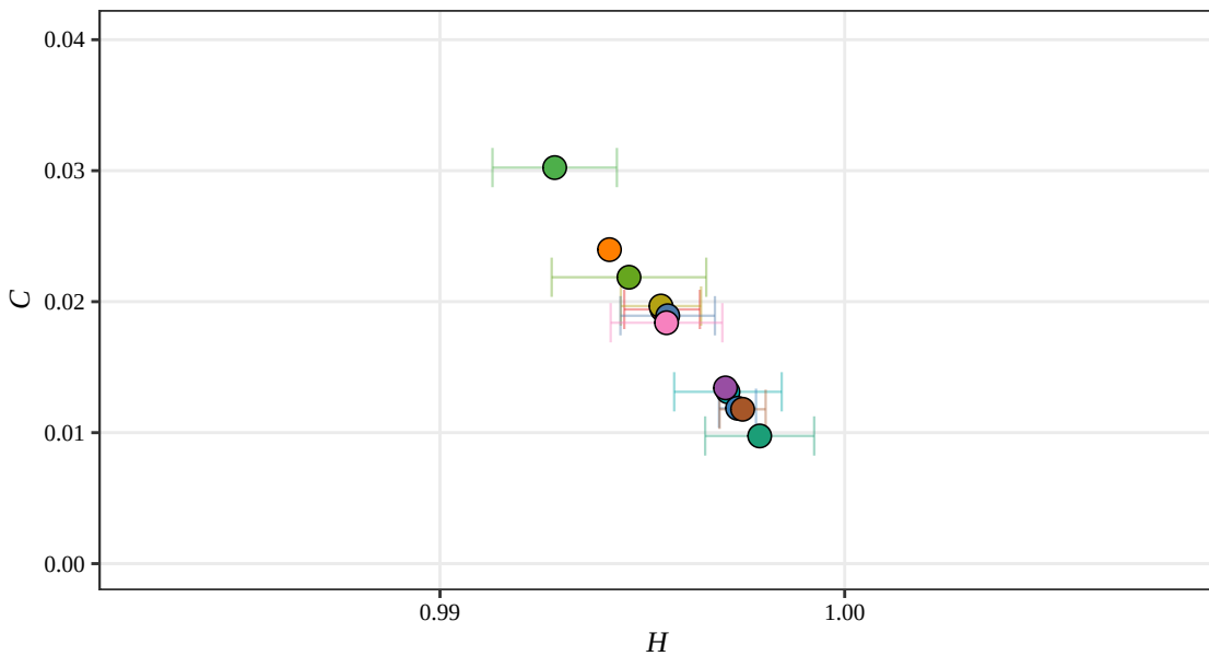
Tsallis H-C Plane, D = 5 (RSAM, 2017)
