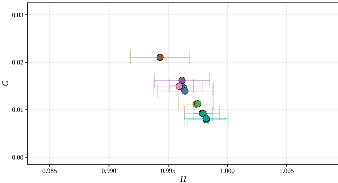
Tsallis H-C Plane, D = 5 (Displacement, 2018)
