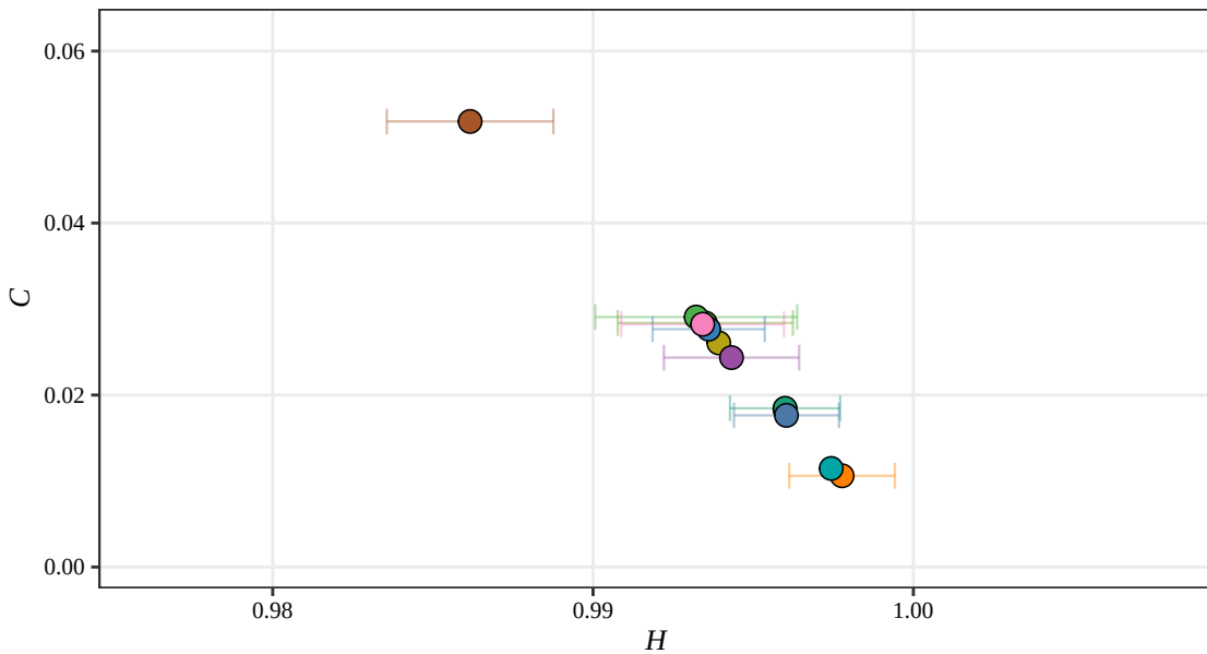
Tsallis H-C Plane, D = 5 (RSAM, 2019)
