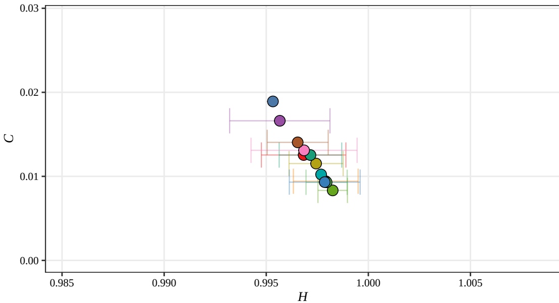
Tsallis H-C Plane, D = 5 (Displacement, 2020)
