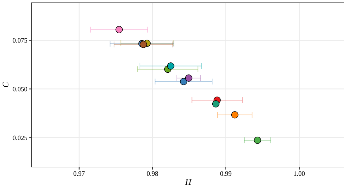
Tsallis H-C Plane, D = 5 (RSAM, 2020)
