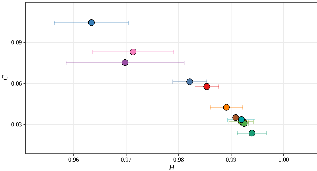
Tsallis H-C Plane, D = 5 (RSAM, 2021)
