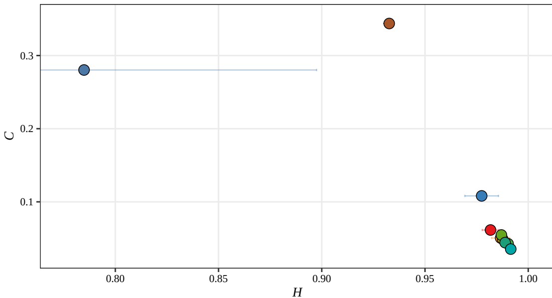
Tsallis H-C Plane, D = 5 (RSAM, 2022)
