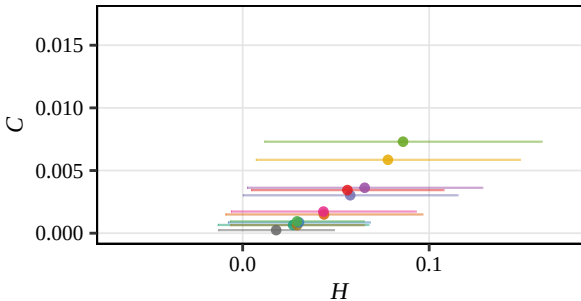
Fisher, D = 5 (RSAM, Apr)
