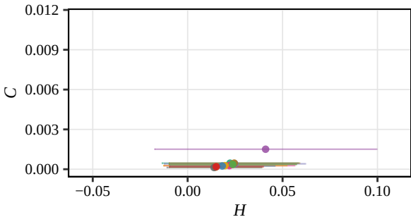
Fisher, D = 5 (Displacement, Jan)
