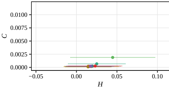
Fisher, D = 5 (Displacement, Mar)
