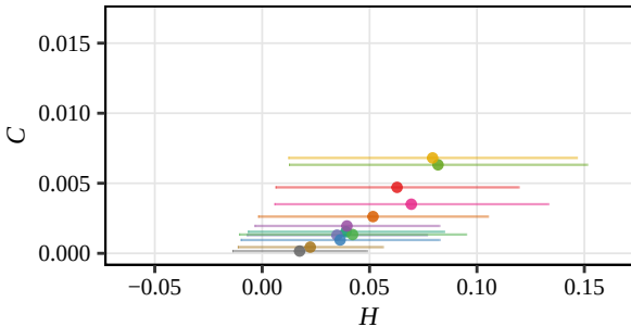
Fisher, D = 5 (RSAM, Mar)
