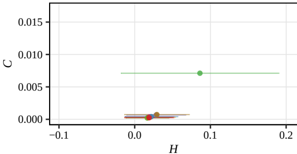
Fisher, D = 5 (Displacement, Nov)
