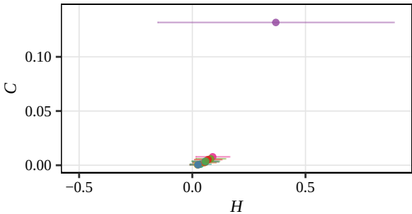
Fisher, D = 5 (RSAM, Sep)
