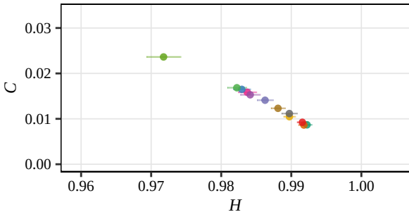
Renyi, D = 5 (Displacement, May)
