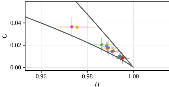
Shannon, D = 5 (Displacement, Apr)
