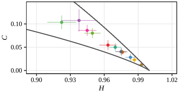
Shannon, D = 5 (RSAM, Aug)
